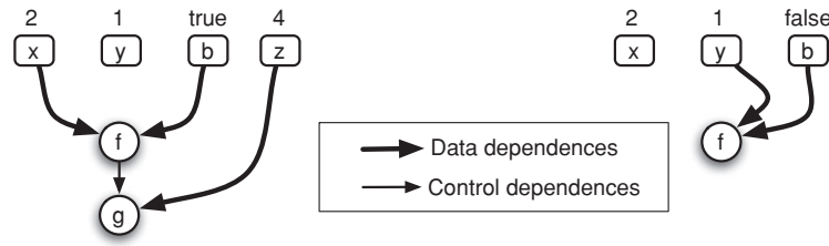
Fig. 1. The DDGs for the simple example.
